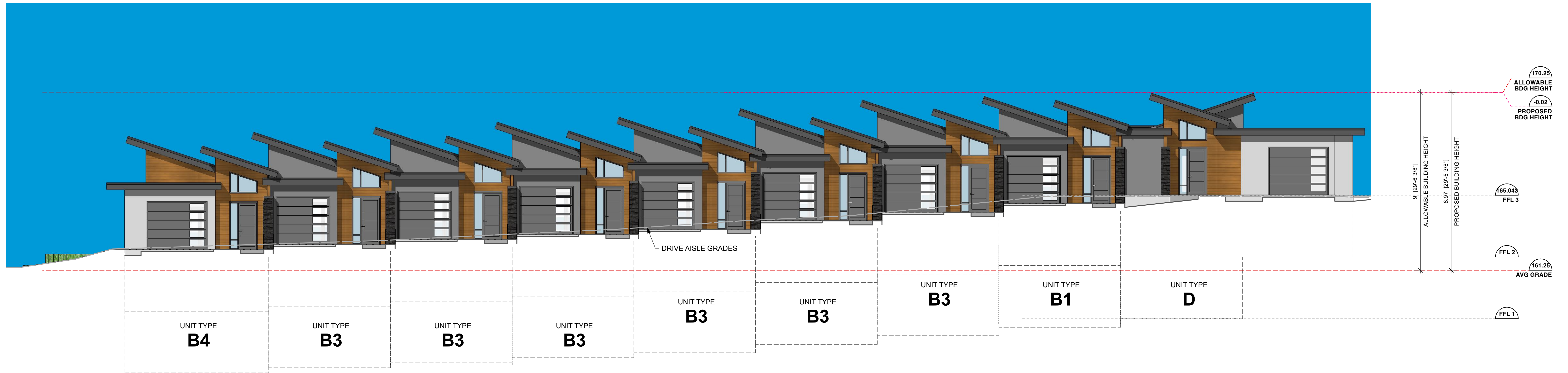
1 Building 12 Street Elevation A315 Scale: 1/8" = 1'-0"
