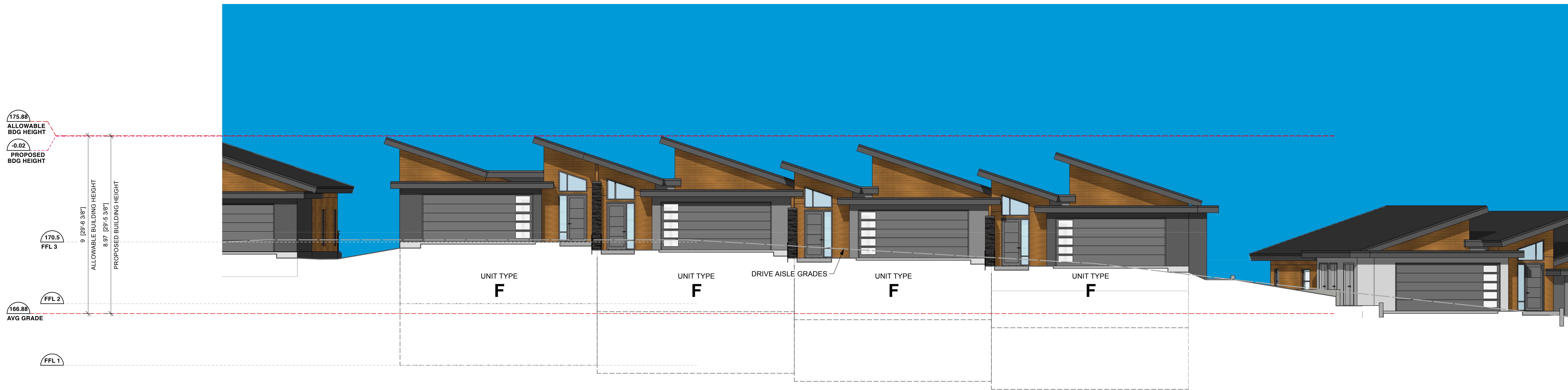
1 Building 3 Street Elevation A311 Scale: 1/8" = 1'-0"
