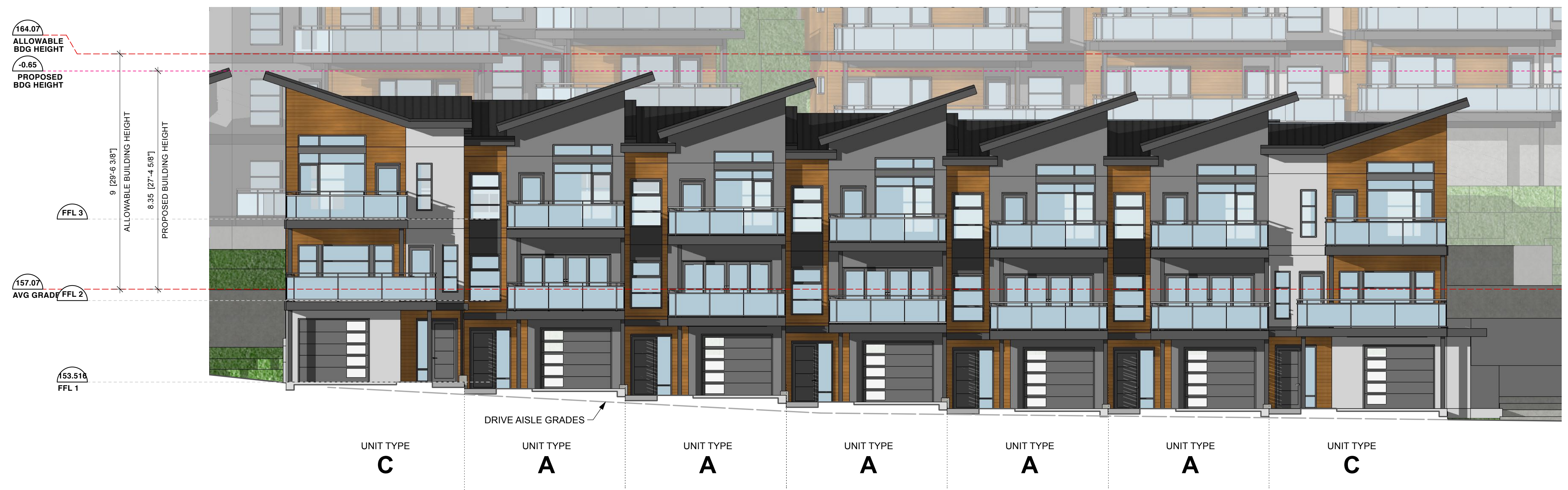
3 Building 7 Street Elevation A312 Scale: 1/8" = 1'-0"
